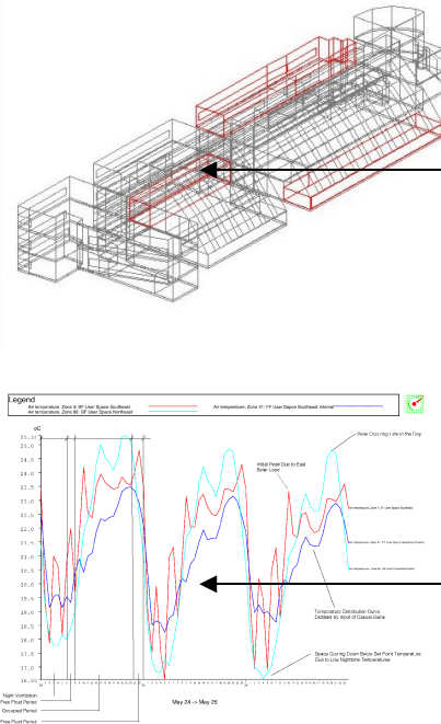
Influence of thermal mass and night cooling
